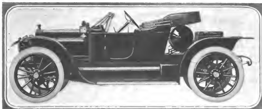
Fig. 9—Side view of the fore-door Rambler with gasoline tank placed behind the driver's seat as well as the trunk with suit cases
